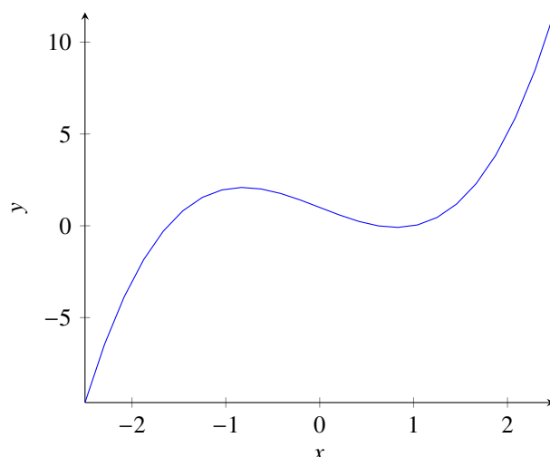
Figure 3.1. Graph of f(x) = x^3 - 2x + 1 .
